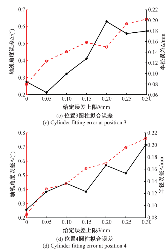
图 9 圆柱拟合后轴线角度误差与圆柱半径误差 Fig. 9 Axis angle error and cylinder radius error after cylindrical fitting
